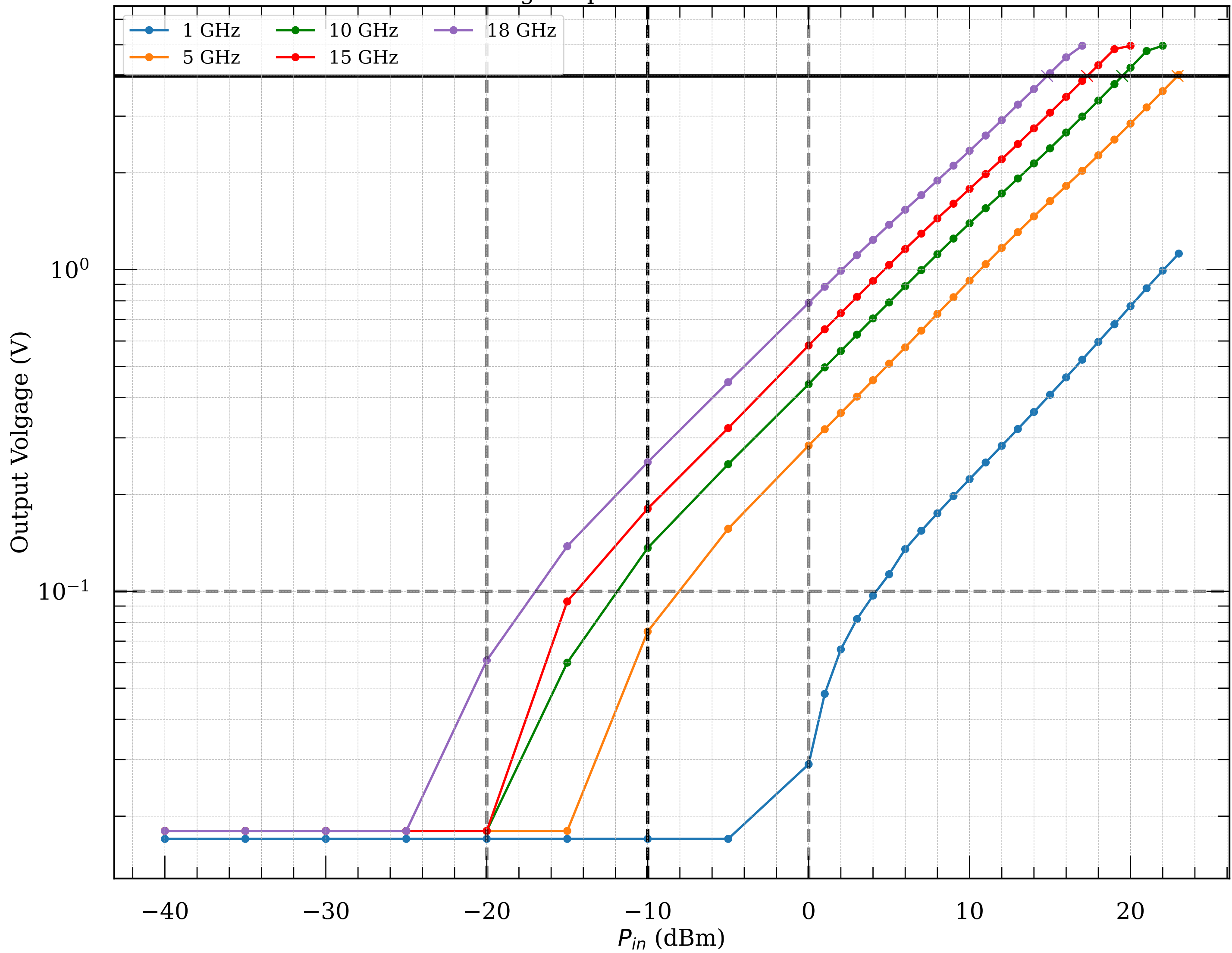
Measured voltage-to-power curve of detector module066
